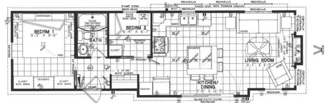
Eastford 25-5244-2TR 43'x12' Escape (538sq.ft.)
