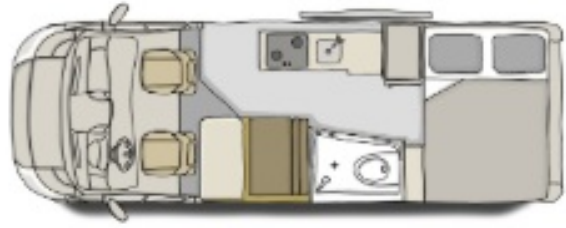
Night floor plan
