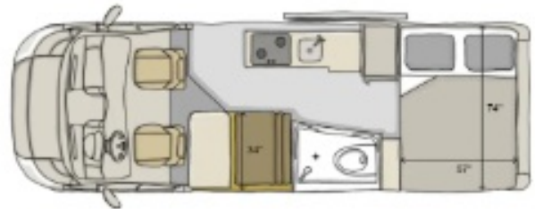
Night floor plan dimensions
