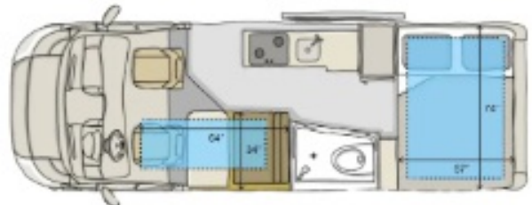
Night floor plan dimensions
