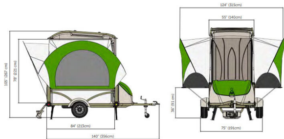
Standard Model
